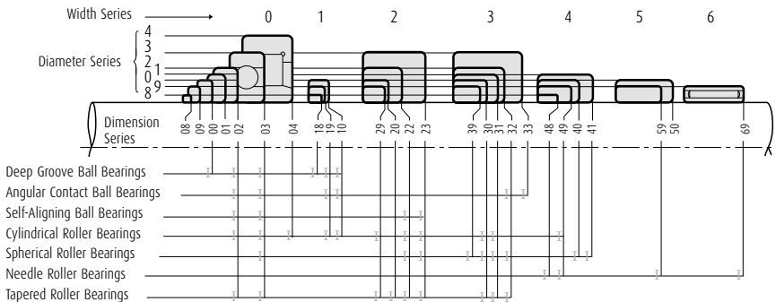
Fig. 2.2 Dimension Series of Radial Bearings
