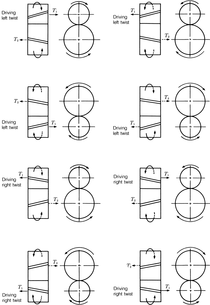
Fig. 4.50 Thrust Direction
