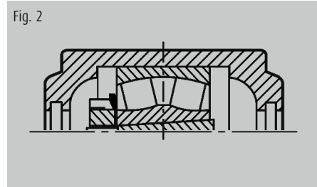
Fig. 2: One bearing should be free to move axially. This plummer block should not be assembled with locating rings.
